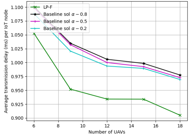
Fig. 13: Evaluation of the transmission delay for the proposed approach LP-F and the baseline solutions LP- \alpha ( \alpha \in \{0.2, 0.5, 0.8\} ) as a function of the number of UAVs.
