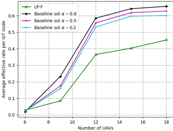
Fig. 12: Evaluation of the effective rate for the proposed approach LP-F and the baseline solutions LP- \alpha ( \alpha \in \{0.2, 0.5, 0.8\} ) as a function of the number of UAVs.
