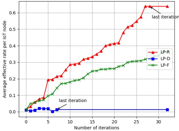
Fig. 6: Evaluation of the effective rate considering LP-R, LP-D and LP-F.
