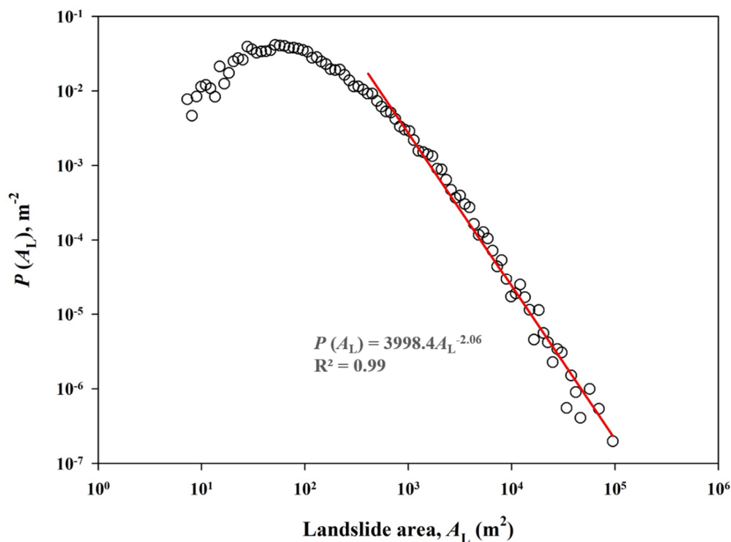
Figure 4. Probability of density distribution for landslide area.
