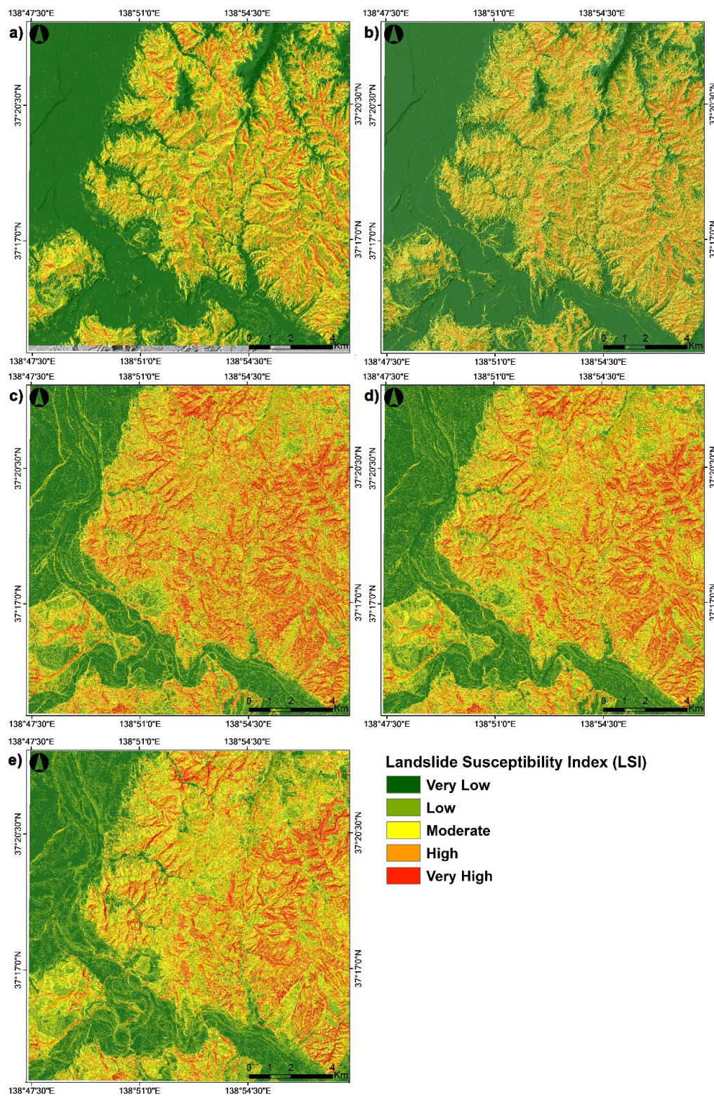
Figure 9. LSM maps produced by (a) PLFR, (b) InV, (c) CF, (d) ANN and (e) SVM models, respectively.
