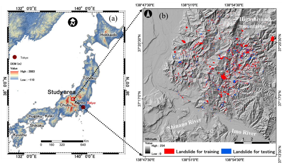
Figure 1. (a) Location of Japan; (b) landslide distribution, randomly divided into two sets: training and testing.
