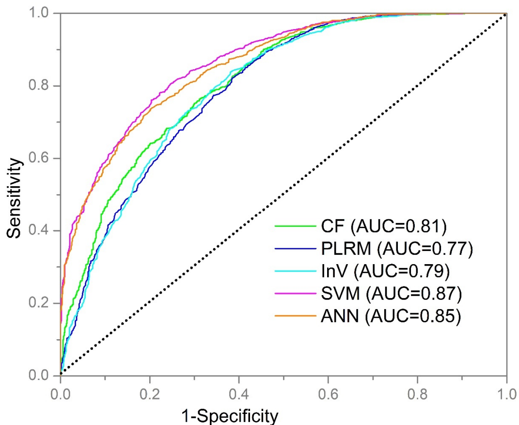
Figure 10. Validation for the performance of five models applying ROC curve in this study.
