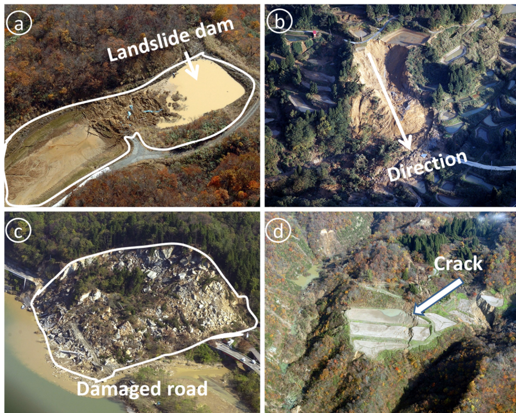
Figure 2. Illustrating the characteristics and different types of landslides in the study area: (a) shallow spread in the north of the Hitotsuminesawa with water, Nagaoka city; (b) rotational soil slide in north of Mushigame; (c) bedrock collapse severely destroyed the road in Nagaoka; (d) translational slide, an arrow display secondary scarp in the Uonuma city (Images provided by NIED).
