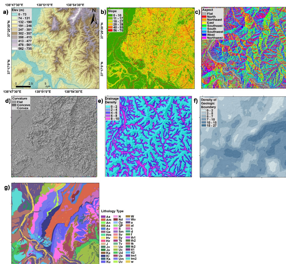
Figure 5. Landslide causative factors maps in this study: (a) elevation, (b) slope angle, (c) slope aspect, (d) plan curvature, (e) drainage density, (f) density of geologic boundaries, (g) lithology.
