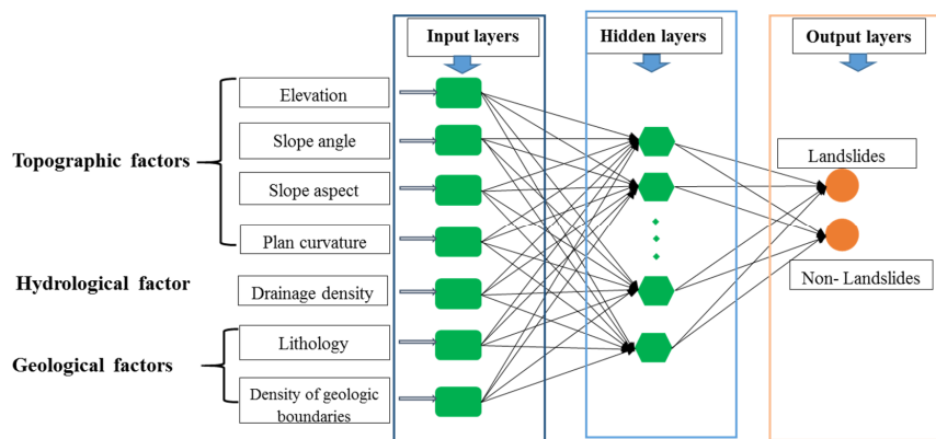
Figure 6. Structure of a three-layer of neural networks for landslide susceptibility analysis.
