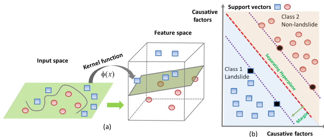
Figure 7. Illustration of support vector machine (SVM) principle: (a) Input space is mapped to the feature space with the help of a kernel function; (b) Separating hyperplane and margin for landslide classification.
