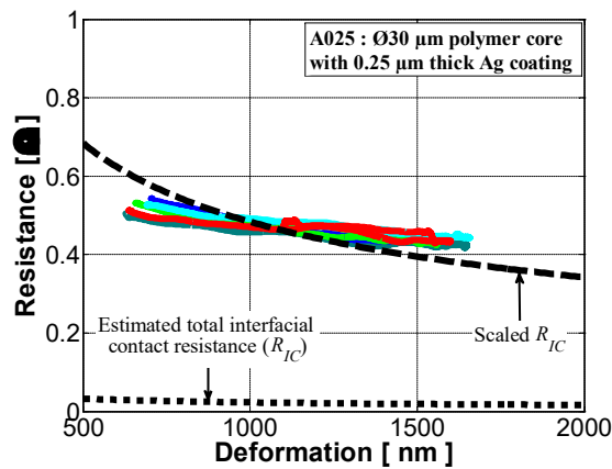
Figure 8: Comparison between total interfacial contact resistance and measured resistances of individual particles as function of particle deformation. Results of A025 particles are selected as an example and shown as solid lines in the figure. The dotted line corresponds to the total interfacial contact resistance ( R_{IC} ) estimated using Eq. (2) and Eq. (3). The dashed line corresponds to R_{IC} being scaled up to the same range as the measured data.
