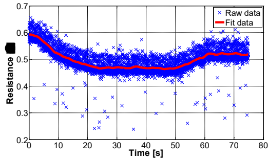
Figure 4: Example of resistance measurement result for an individual AgPS from group A020; raw data vs. fit data. The root mean squared deviation of the data fitting is about 0.026 \Omega .
