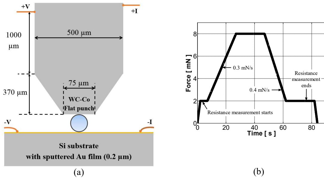
Figure 2: Experimental setup for the electrical measurements of individual particles using a nanoindentation-based flat punch test (a), and loading profile of all indentation tests (b). The drawing for the experimental setup is not to the scale. The period of the electrical measurements is indicated in Figure 2b.
