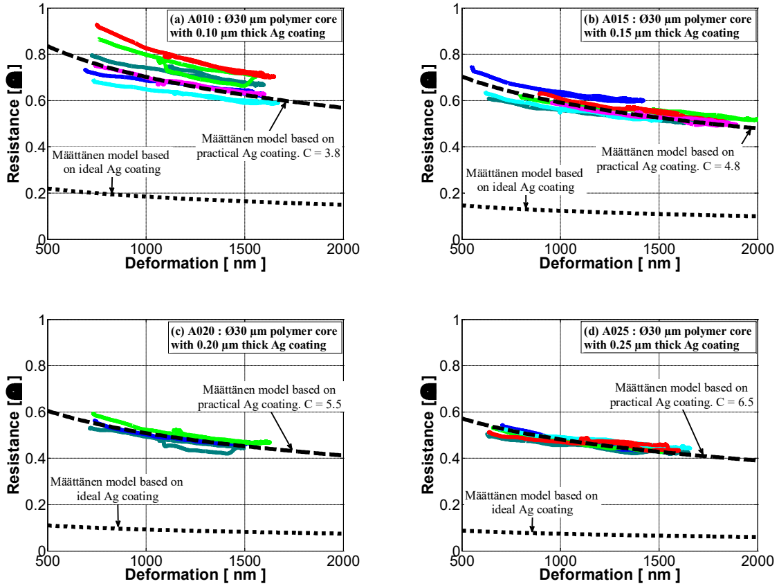
Figure 9: Comparison between experimental results and theoretical models for the four groups of AgPS. In each graph, the solid lines correspond to the measured resistance-deformation curves of individual particles shown in Figure 6; the dotted line corresponds to the Määttänen model based on ideal Ag coating (Eq. (4)); and the dashed line corresponds to the Määttänen model based on practical Ag coating with parameter C specified in Eq. (5).
