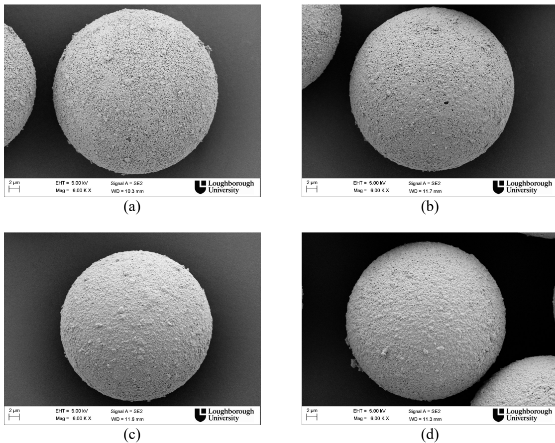
Figure 1: SEM images of particles consisting of Ø30 μm polymer spheres coated with (a) 0.10 μm thick (A010), (b) 0.15 μm thick (A015), (c) 0.20 μm thick (A020) and (d) 0.25 μm thick (A025) Ag coating.
