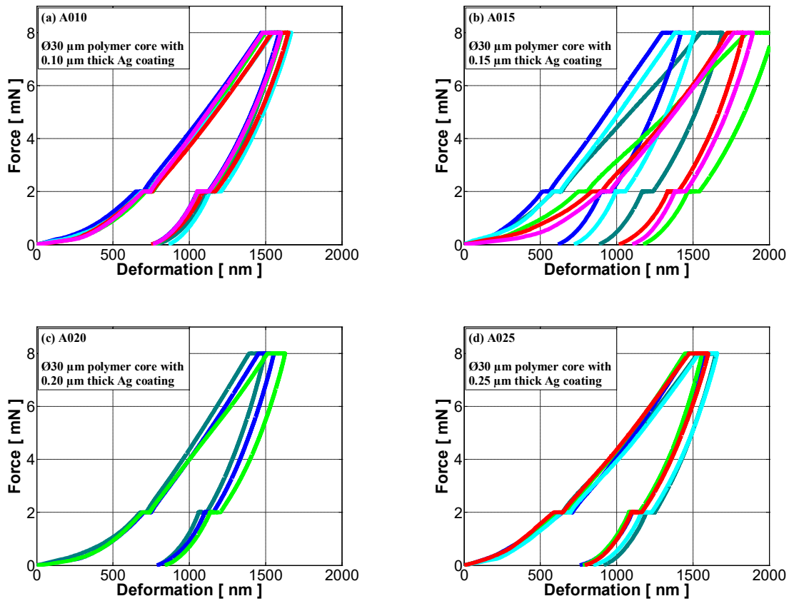
Figure 3: Indentation force-deformation curves for the four groups of AgPS. Each curve in a graph presents measurement result of an individual particle from the corresponding group. The plateaus in each force-deformation curve are corresponding to the holding segments on the loading profile, where applied force is held constant at 2 mN, 8 mN and then 2 mN (Figure 2b). The loading rate from 2mN to 8 mN and the unloading rate from 8 mN to 2 mN are 0.3 mN/s and 0.4 mN/s, respectively.
