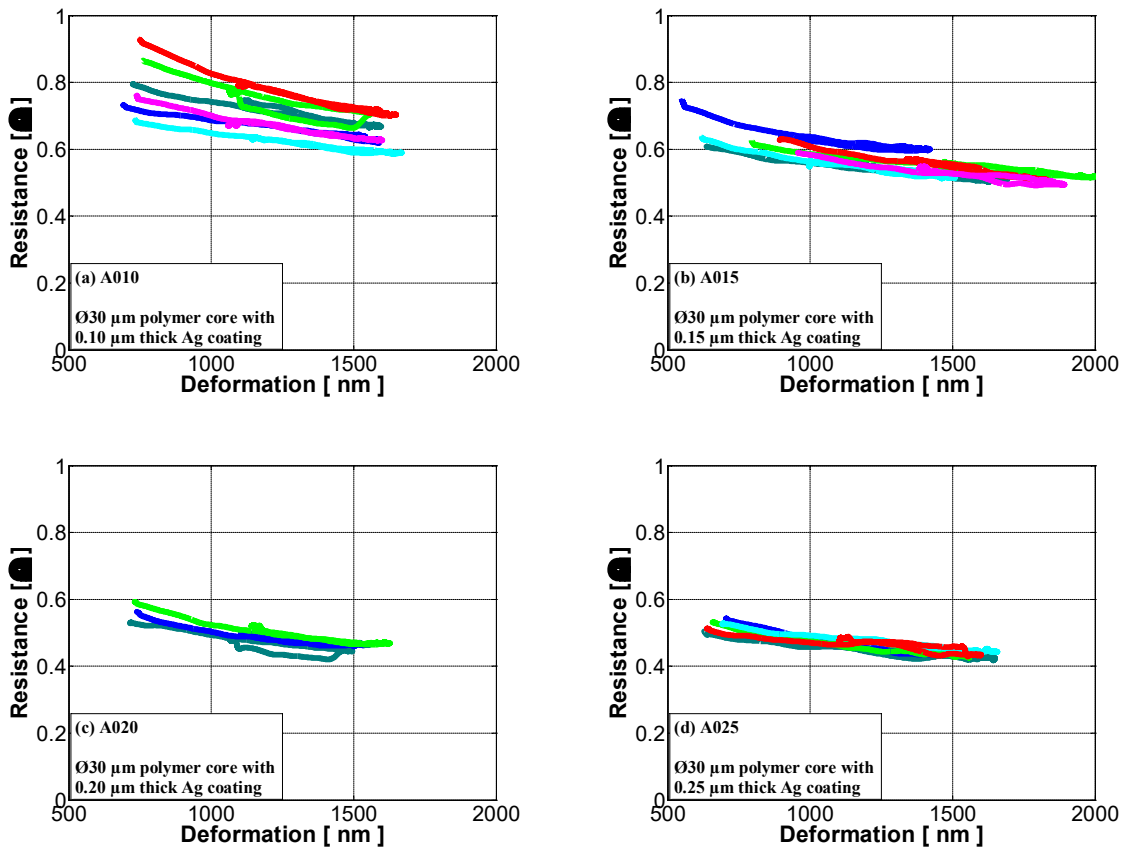
Figure 6: Measured resistance-deformation curves for the four groups of AgPS. Each curve in a graph presents measurement result of an individual particle from the corresponding group.
