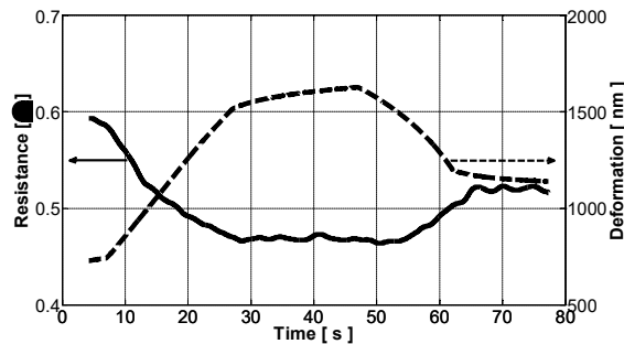
Figure 5: Example of electrical resistance and corresponding deformation of an individual AgPS from group A020 as function of time.
