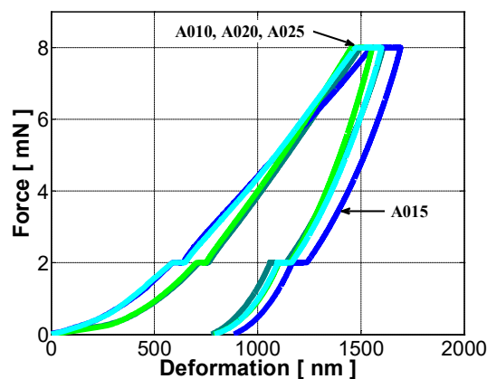
Figure 7: Comparison of mechanical response for the four groups of AgPS tested. The force-deformation curve corresponding to each group of particles is represented by the median curve (see Figure 3).
