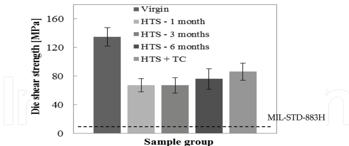
Figure 9. Die shear strength for virgin Au-Sn SLID samples, high-temperature-stored (HTS) samples—at 250°C for 1, 3 and 6 months—and samples exposed for 3 months HTS + 1000 thermal cycles (TC) between 0 and 200°C. Reprinted with permission from Springer Nature [23].
