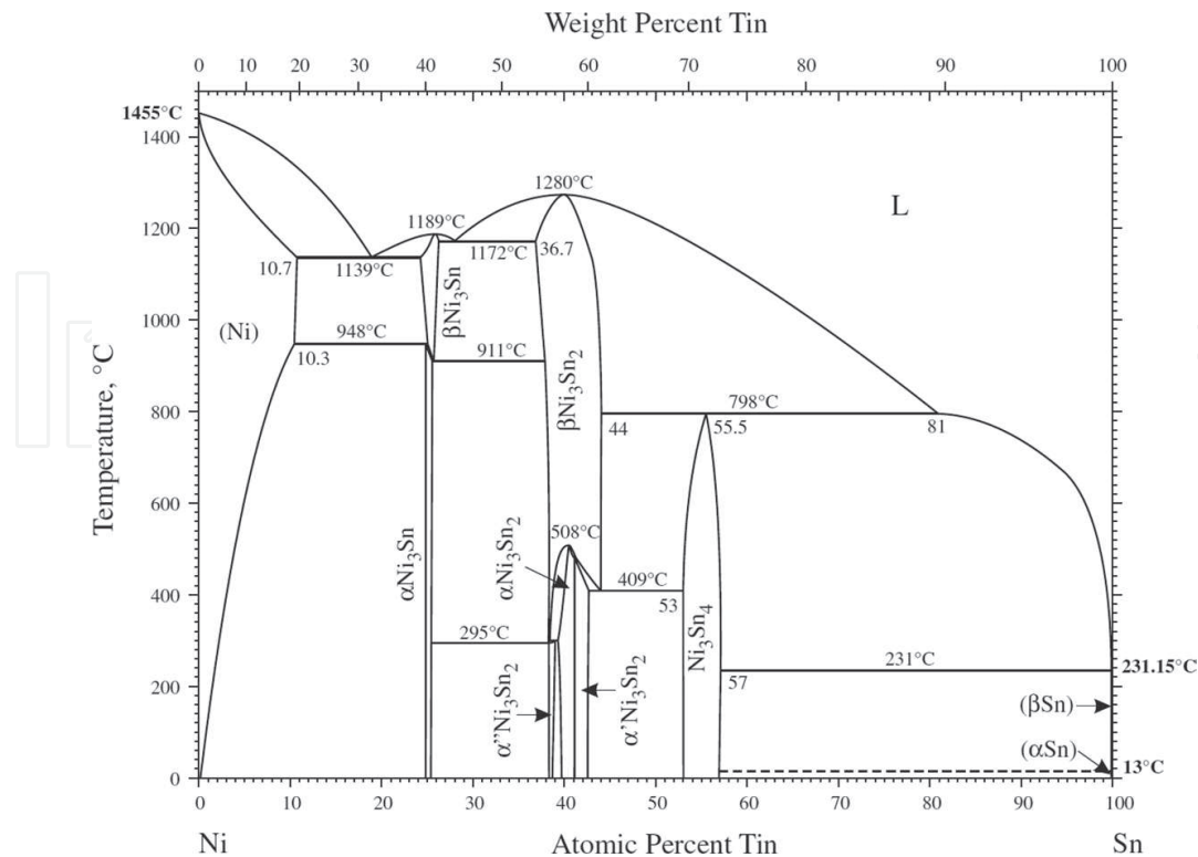
Figure 10. Ni-Sn phase diagram. Reprinted with permission from Springer Nature [24].
