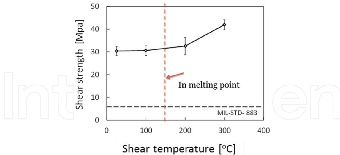
Figure 15. Au-In strength versus temperature.
