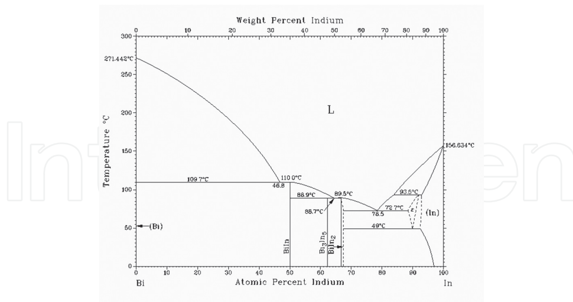
Figure 16. The Bi-In phase diagram. Reprinted with permission from ASM International [37].
