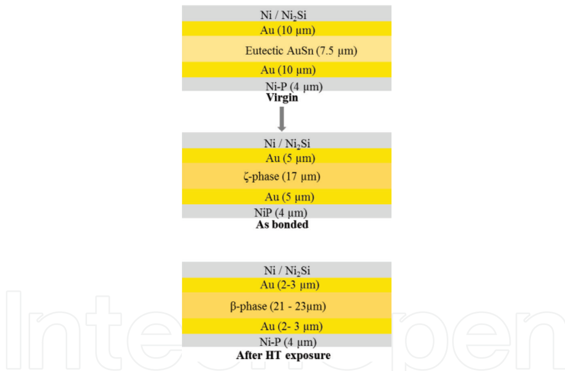
Figure 8. A schematic overview of the layered structure of an optimized Au-Sn SLID bond at different life stages. The different material phases were identified with energy-dispersive X-ray spectroscopy (EDX) and X-ray diffraction. Reprinted with permission from Springer Nature [23].
