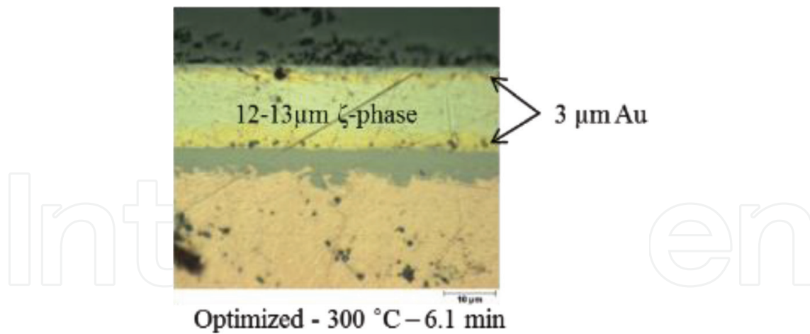
Figure 7. Cross section of an optimized Au-Sn SLID bond [22] (© 2012 IEEE).
