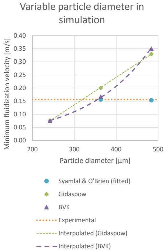
Figure 7. Minimum fluidization velocity from simulations using particle diameters 242, 363 and 484 μm.
