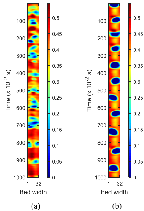
Figure 11. ECT images for 10 s of the flow in bed of 483 μm sand particles at 31 cm/s: (a) lower plane: 15.7 cm from the bottom (b) upper plane: 28.7 cm from bottom. Time axis increases from top to bottom.
