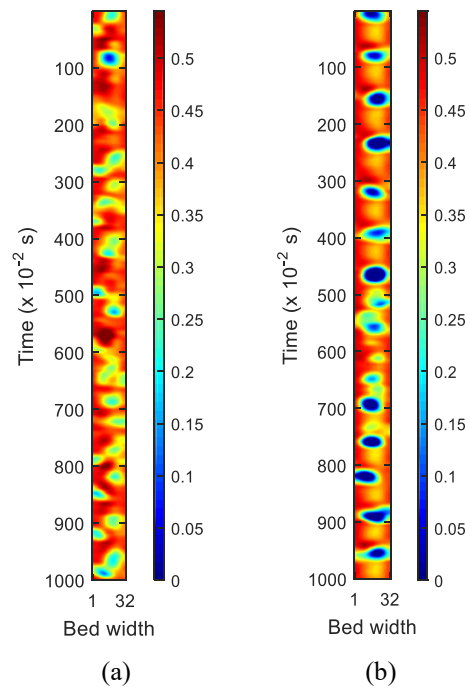
Figure 10. ECT images for 10 s of the flow in bed of 483 μm sand particles at 25 cm/s: (a) lower plane: 15.7 cm from the bottom (b) upper plane: 28.7 cm from bottom. Time axis increases from top to bottom.
