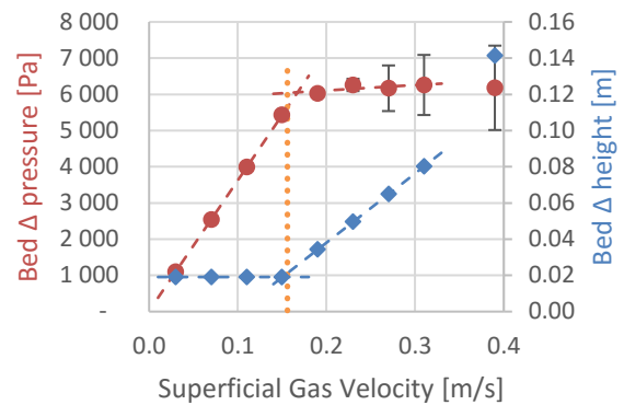
Figure 6. Bed pressure drop (red-left) and bed height increase (blue-right) from simulation using BVK drag model, particle diameter 363 \mu\text{m} . Error bars indicate variation due to bubbles. Dotted line marks the experimental minimum fluidization velocity.
