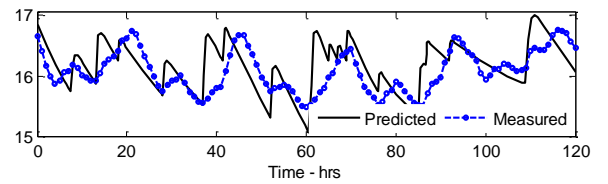
Figure 4: Variation of inside air temperature in the single-zone model [°C].
