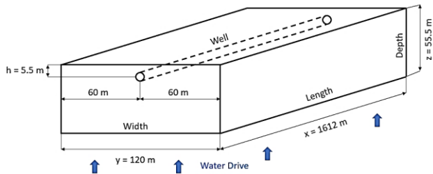
Figure 6: Schematic geometry of the drainage area.
