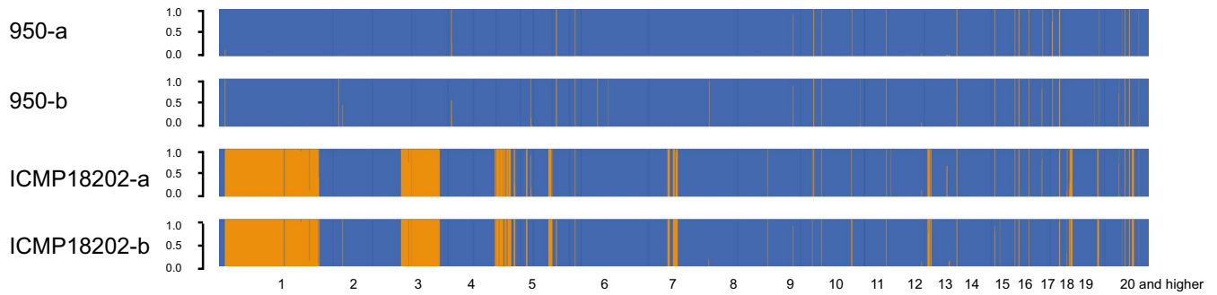
FIGURE 5 The genomic assignment of the two isolates of Serpula lacrymans from New Zealand (950 and ICMP18202) to the European and Japanese populations estimated with PCADMIX. The analyses are done along the genome of the European S. lacrymans S7.3, for genomic windows of 10 SNPs, where the numbers on the x-axis represent the scaffold numbers. Strain ID-a and -b indicate the two different haplotypes after phasing the SNPs from the dikaryotic strains using BEAGLE. Blue indicates genomic windows assigned to the European population, while yellow indicates genomic windows assigned to the Japanese population
