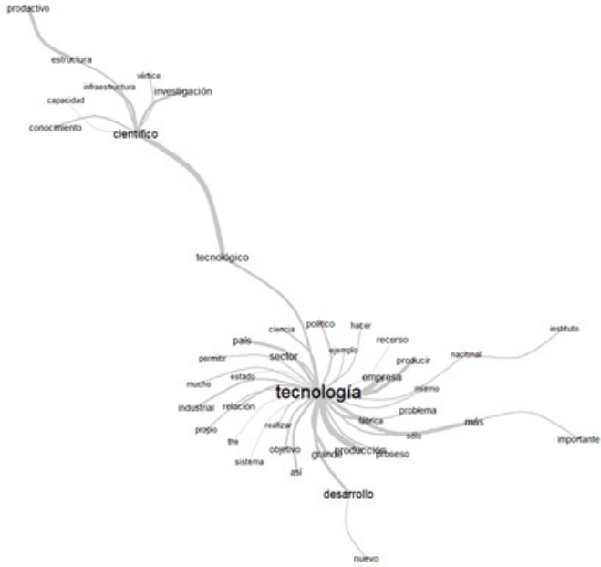
Figure 4: Similitude analysis of Sábató's Triangle.
