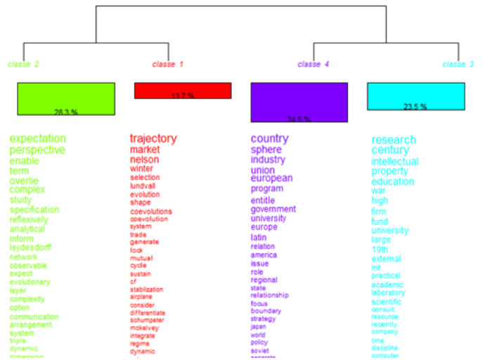
Figure 5: Dendrogram of the Triple Helix.
