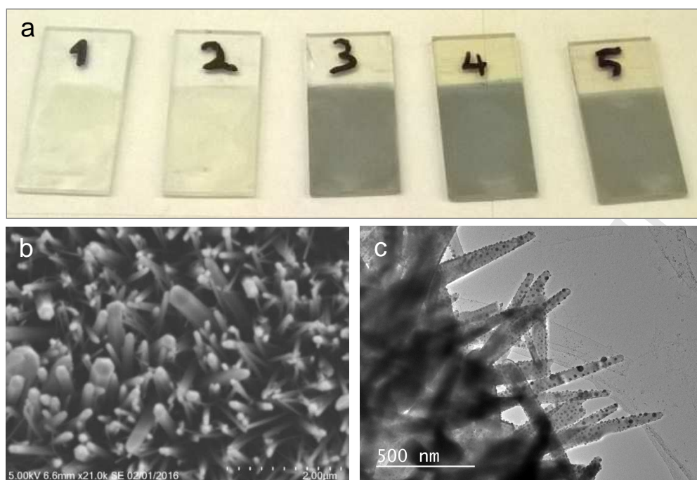
Fig. 2. a) A photograph of the resulting samples of ZnO, ZnO-SiO 2 , ZnO-Au, ZnO-SiO 2 -Au, ZnO-Au-SiO 2 , corresponding to the samples in Figure 1, b) and c) SEM images of ZnO nanorods with Au and SiO 2 deposition.
