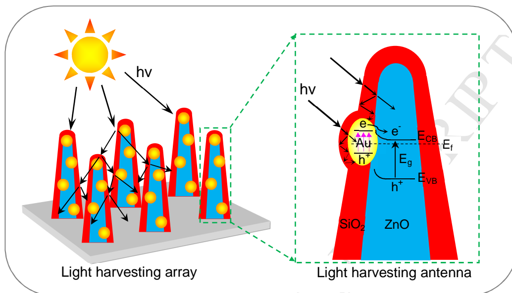
Fig. 6. Light harvesting mechanisms and photoelectrical physics.
