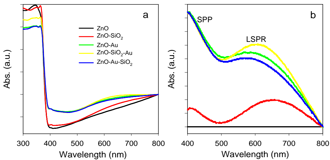
Fig. 4. a) UV-vis absorption spectra of the nanorods with and without coating, b) the absorption spectra by subtracting the spectra of ZnO.
