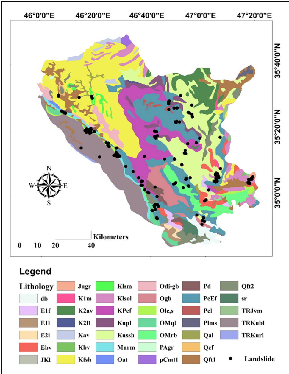
Figure 3. The lithology of the study area.
