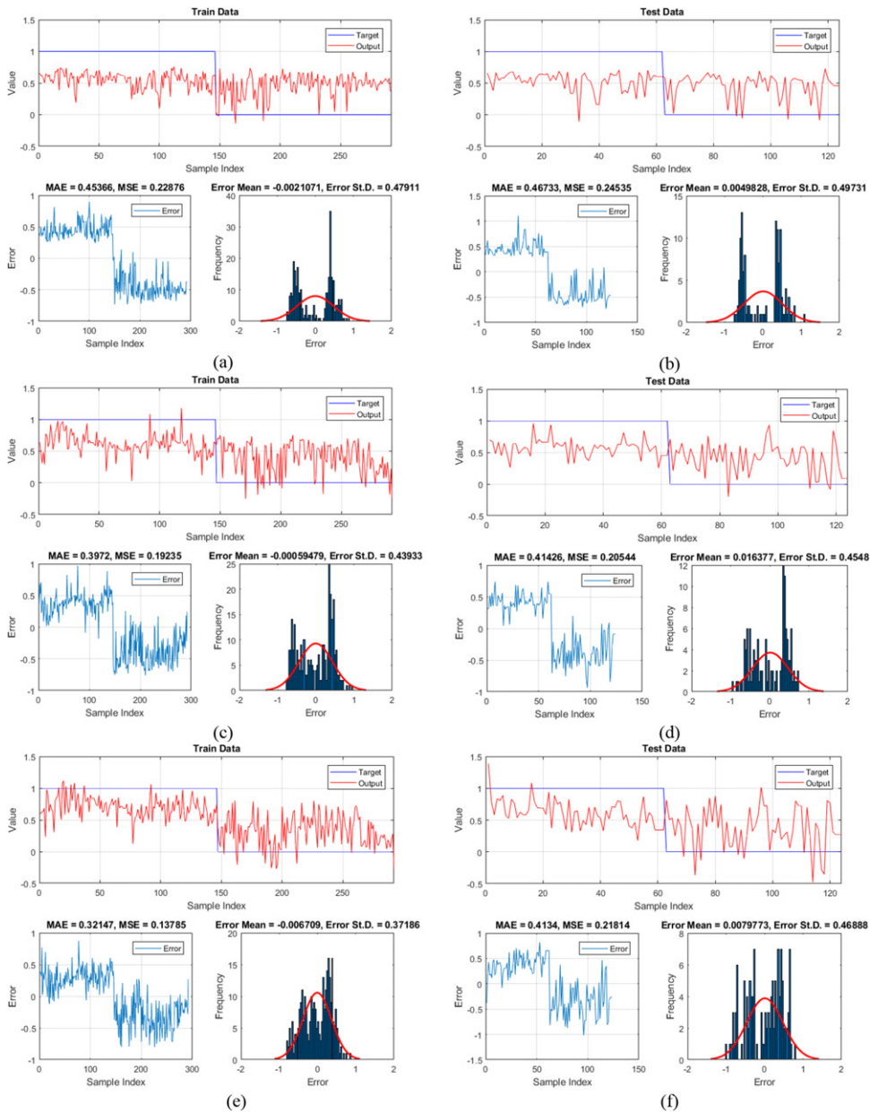
Figure 10. The results obtained for the (a and b) MLP, and (c and d) DA-MLP, and (e and f) BBO-MLP, respectively for the training and testing samples.
