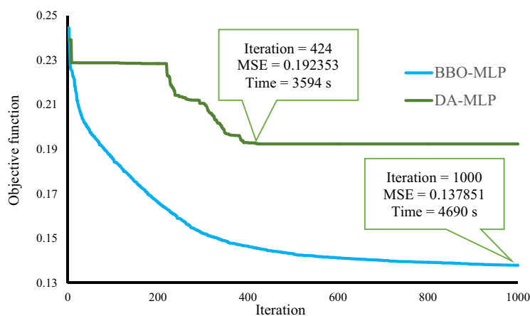
Figure 8. The convergence cure of the applied DA-MLP and BBO-MLP models.
