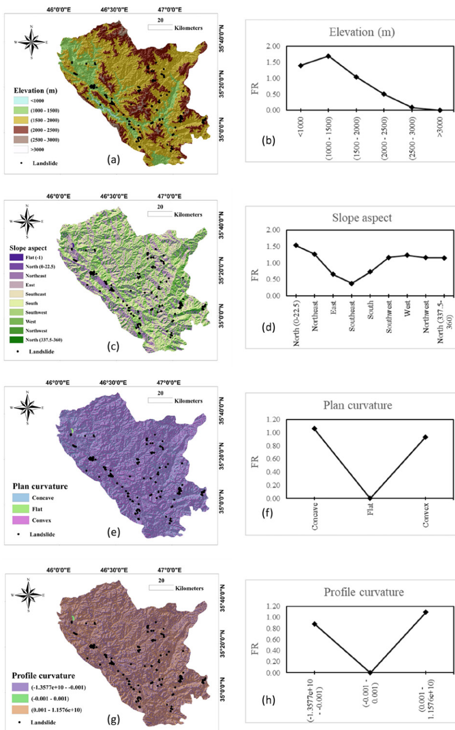
Figure 2. The calculated FR for: (a and b) elevation, (c and d) slope aspect, (e and f) plan curvature, (g and h) profile curvature, (i and j) soil type, (k and l) distance to river, (m and n) distance to road, (o and p) distance to fault, (q and r) land cover, (s and t) slope degree, (u and v) SPI, (w and x) TWI, and (y and z) rainfall.
