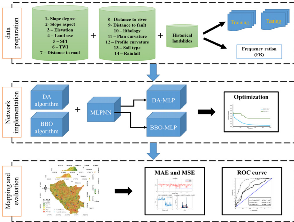
Figure 4. Applied procedure for landslide susceptibility assessment of this study.
