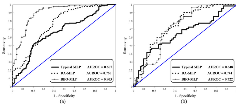
Figure 11. The ROC curves plotted for the (a) training and (b) testing datasets.
