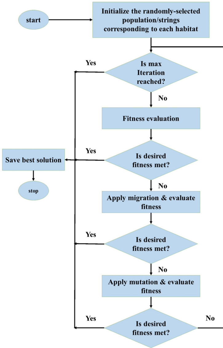
Figure 7. The flowchart of the BBO algorithm.
