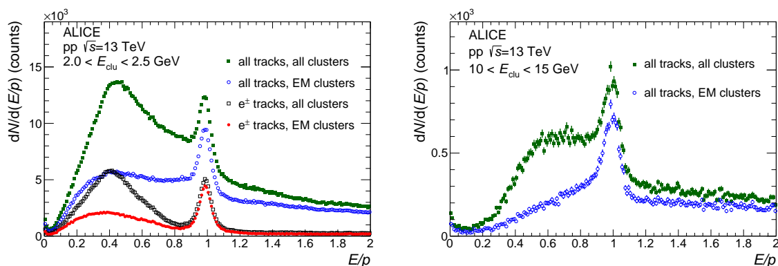
Figure 10. [Color online] Distribution of the cluster energy to track momentum, E/p ratio, for two ranges of cluster energies E_{\text{clu}} in one PHOS module. A peak around unity due to the electron contribution is visible.
