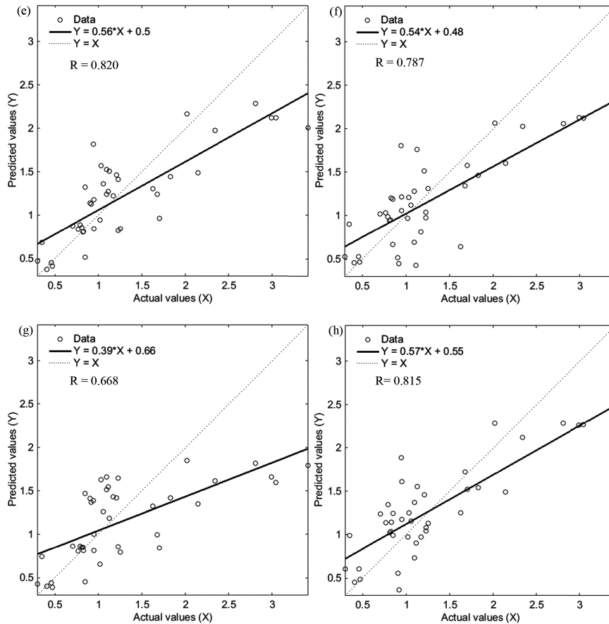
Fig. (5). Analysis of correlation between actual and predicted Cv values using the models: (a) Model 1, (b) Model 2, (c) Model 3, (d) Model 4, (e) Model 5, (f) Model 6, (e) Model 7, (h) Model 8.
