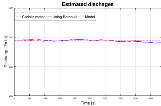
Figure 11: Flow estimation of a single data set
