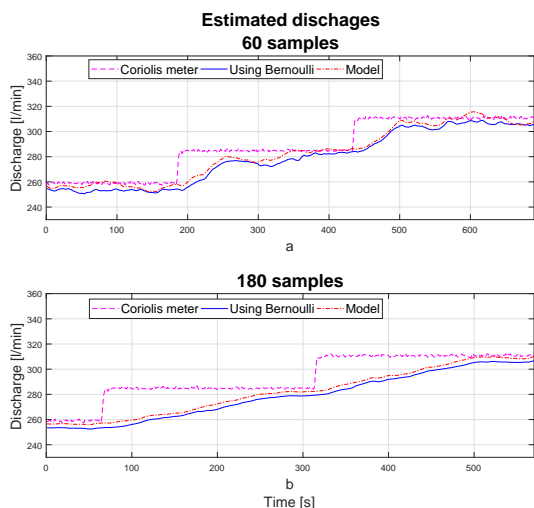
Figure 12: Flow estimation after a step change
