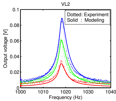
Figure 4. Output voltage at transducer 2 for acceleration amplitude of 0.01\text{ g} (linear regime) and bias voltage of 30\text{ V} , 20\text{ V} and 10\text{ V} (top to bottom)
