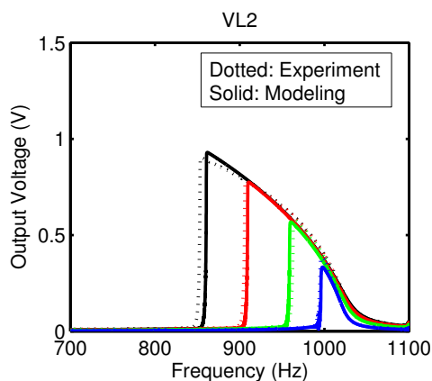
Figure 8. Output of transducer 2 with 11^{th} order polynomial damping force for acceleration amplitudes of 0.28 g , 0.25 g , 0.19 g , 0.1 g (left to right), bias voltage of 20 V .
