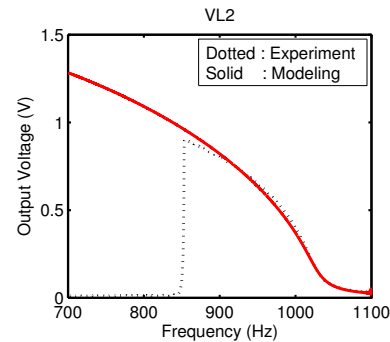
Figure 5. Output voltage at transducer 2 for acceleration amplitude of 0.28\text{ g} (nonlinear regime) and bias voltage of 20\text{ V} .
