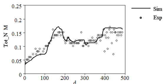
Figure 7: Simulated and experimental total ammonia concentration
