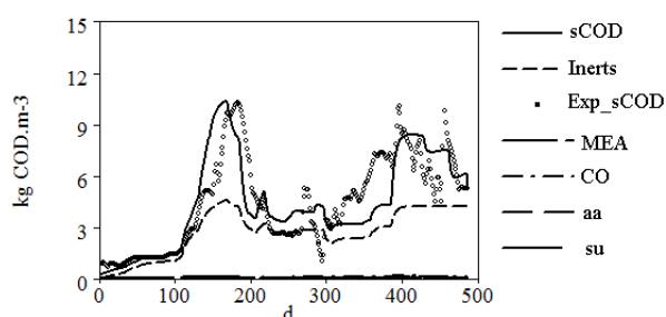
Figure 4: Simulated and experimental effluent components concentrations (COD based). aa, amino acid; su, monosaccharides
