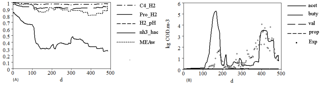
Figure 5: Simulated inhibition effects (A) from H 2 on butyrate and propionate degradation (C4_H2 and Pro_H2), pH effects on hydrogen degradation (H2_pH) and NH_3 and MEAw effects on acetate degradation (nh3_hac and MEAw) in AD of MEAw. VFA accumulation (B), acet, acetate; buty, butyrate; val, valerate; prop, propionate
