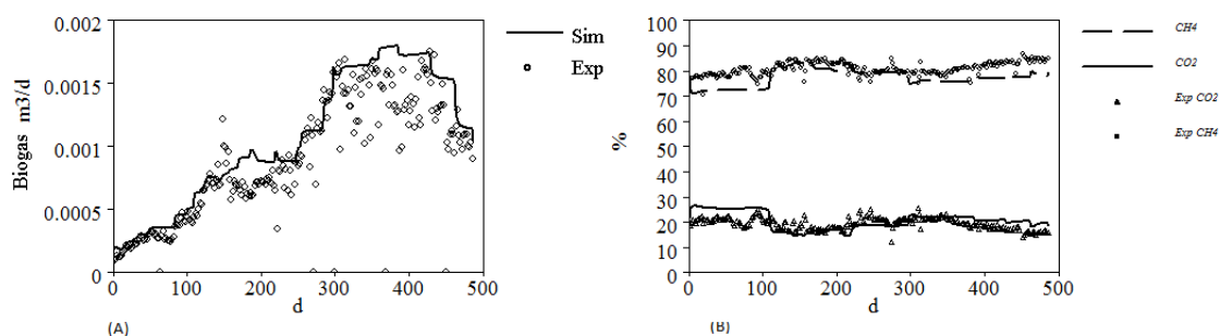
Figure 8: Simulated and experimental biogas generation (A) and CH_4 and CO_2 partial pressures (B)
