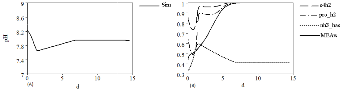
Figure 3: Simulated pH (A) and inhibition effects (B), c4h2, pro_h2, nh3_hac and MEAw are inhibitions of hydrogen on butyrate, propionate degradation, free ammonia and MEAw on acetate degradation, respectively
