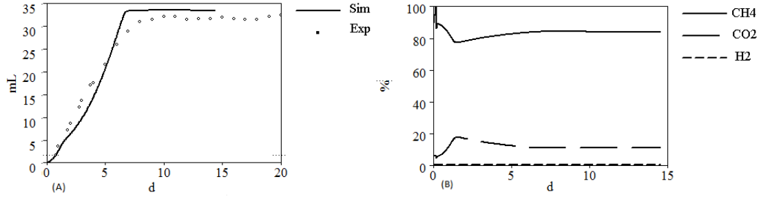
Figure 2: Biogas accumulation (A) and partial gas pressure (B) simulated by the extended model
