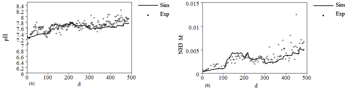
Figure 6: Simulated and experimental pH (A) and free ammonia concentration (B)
