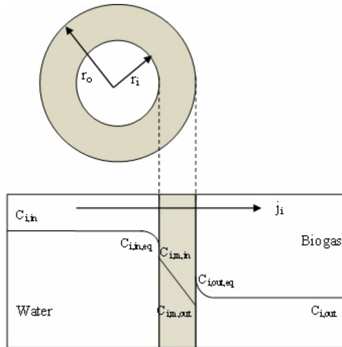
Figure 2. Distribution of oxygen and nitrogen concentration gradients
