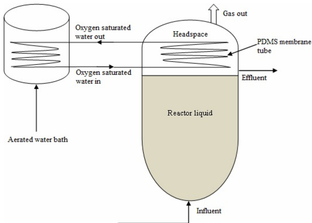
Figure 1. Arrangement of the mass transfer membrane loop inside the digester using an aerated water bath to supply oxygen to the circulating water
