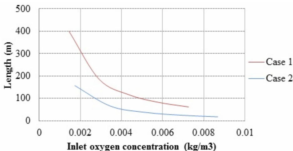
Figure 4. Calculated required membrane length vs. Velocity for the two cases ( r_{im} = 4.5 mm)
