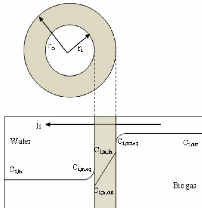
Figure 3. Distribution of methane, carbon dioxide and hydrogen sulfide concentration gradients
