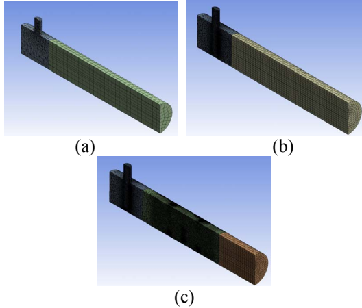
Figure 3. Mesh cross sectional view; (a) Case-1, (b) Case-2, (c) Case-3
