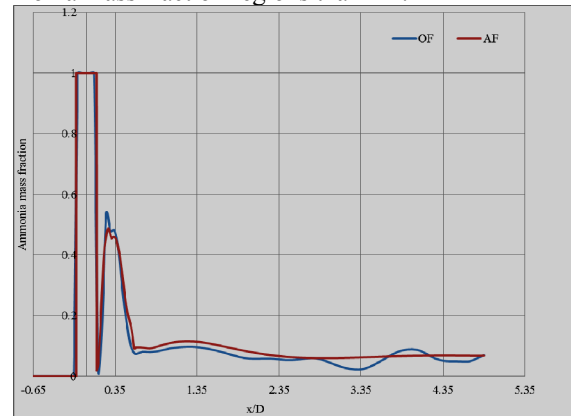
Figure 7. Ammonia mass fraction along central axis – case2
