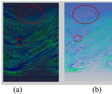
Figure 16. Large and small eddies (large circles and small circles show large eddies and small eddies respectively): (a) OF, (b) AF
