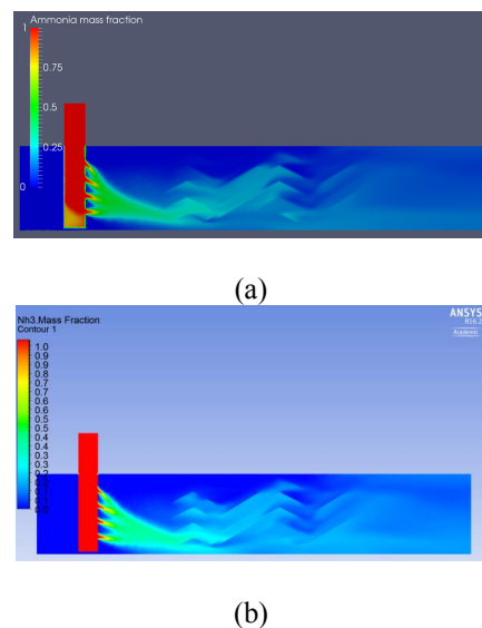
Figure 8. Ammonia mass fraction case-3; (a) OF, (b) AF
