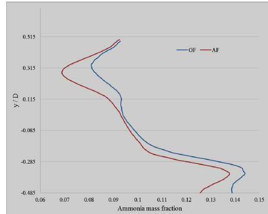
Figure 11. Ammonia mass fraction along the vertical lines at x/D = 4.85 (y negative is below the center of plane and vertical lines are shown in Fig.10)
