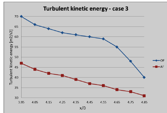
Figure 12. Turbulent kinetic energy comparison – case 3 (Average turbulent kinetic energy in mixing evaluation planes)
