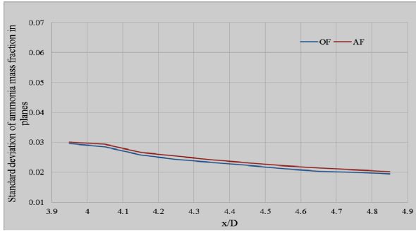
Figure 9. Mixing evaluation - case 3 (standard deviation of ammonia mass fraction)
