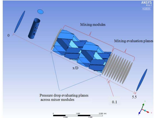
Figure 4. Mixing evaluation planes
