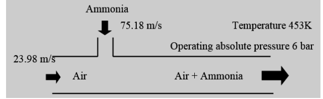
Figure 1. Air and ammonia inlets, outlet and flow directions
