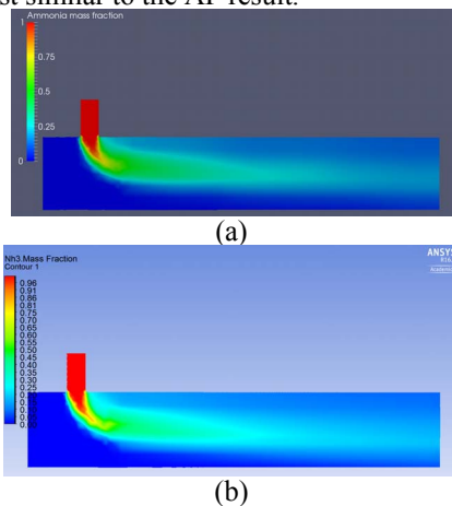
Figure 5. Ammonia mass fraction contours case -1; (a) OF, (b) AF
