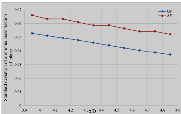
Figure 6. Mixing evaluation – case1 (standard deviation of ammonia mass fraction)
