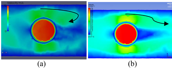
Figure 15. Vortex street comparison – Velocity contours around ammonia injecting pipe; (a) OF, (b) AF
