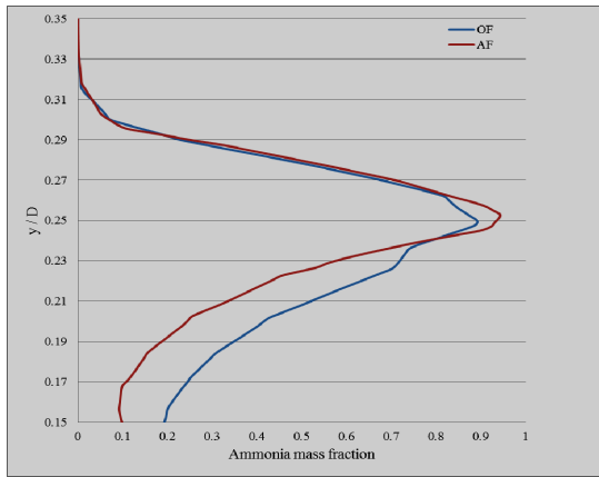
Figure 14. Ammonia mass fraction across a jet (mass fractions were plotted along the verticle lines those lines are shown in Fig.13)
