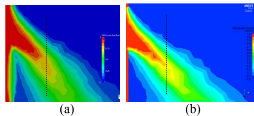
Figure 13. Jet mixing at first hole in injector; (a) OF, (b) AF
