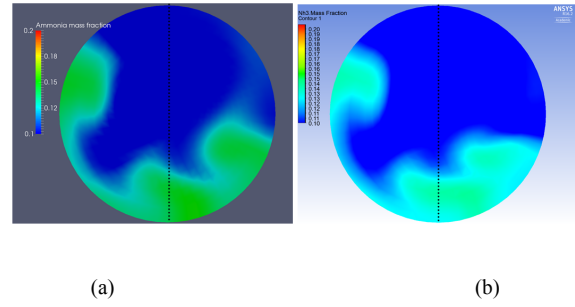
Figure 10. Ammonia mass fraction contours at x/D = 4.85 ; (a) OF, (b) AF
