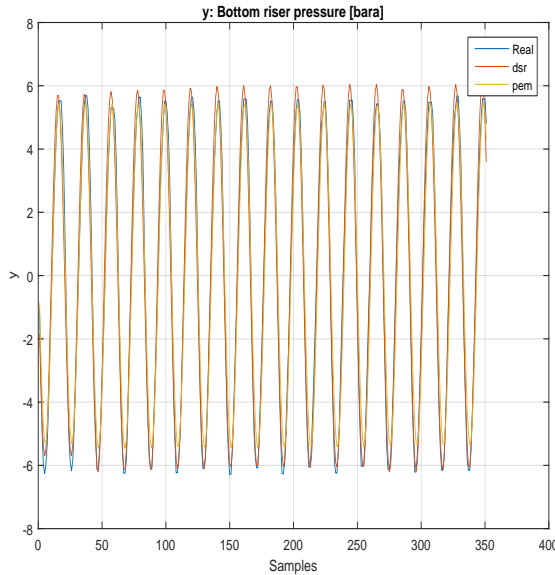
Figure 16: Illustration of the identified models simulated over the unused part of the validation set. We have V_{DSR_8^s} = 0.3932 V_{PEM} = 0.5039 . See Fig. 13. for details.
