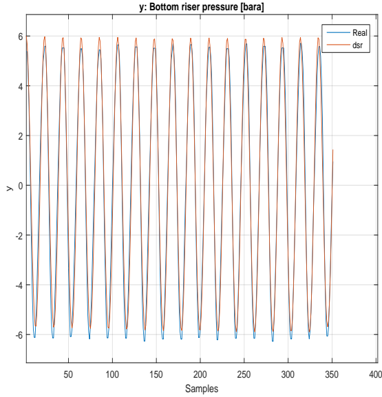
Figure 15: Identified model DSR_8^s (Eq. 18) simulated over the identification set. This figure shows simulation from 500 to 850 samples in Fig. 14.
