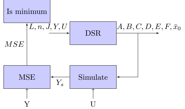
Figure 3: Block diagram of the proposed members working together through iterations of L, n, J , each bounded as described in Eq. 8. The optimal model, meaning the model giving the lowest MSE, is chosen. The ‘DSR’ block is as Eq. 7 and the ‘MSE’ block is as Eq. 9.
