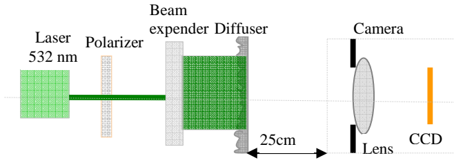
Fig. 1 Experimental setup
